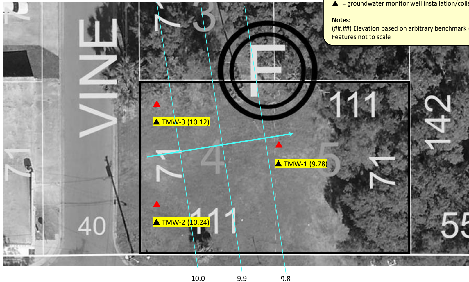
Figure 4 Shallow Groundwater Elevation Map (04/21/2023)
